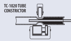
TC-1020 TUBE CONSTRICTOR FILL WITH SOLDER Joint is ready for sweating when constricted tube contacts smaller tube. Can be used for crimping applications.
