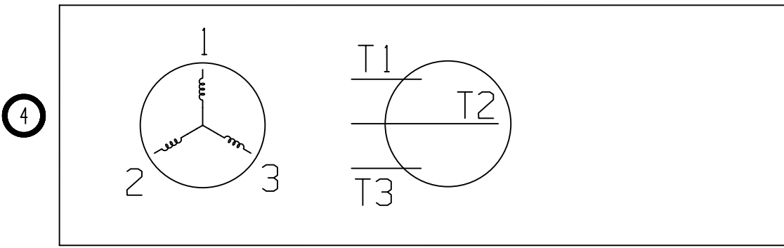
COMPRESSOR WIRING DIAGRAM THREE PHASE MOTOR
