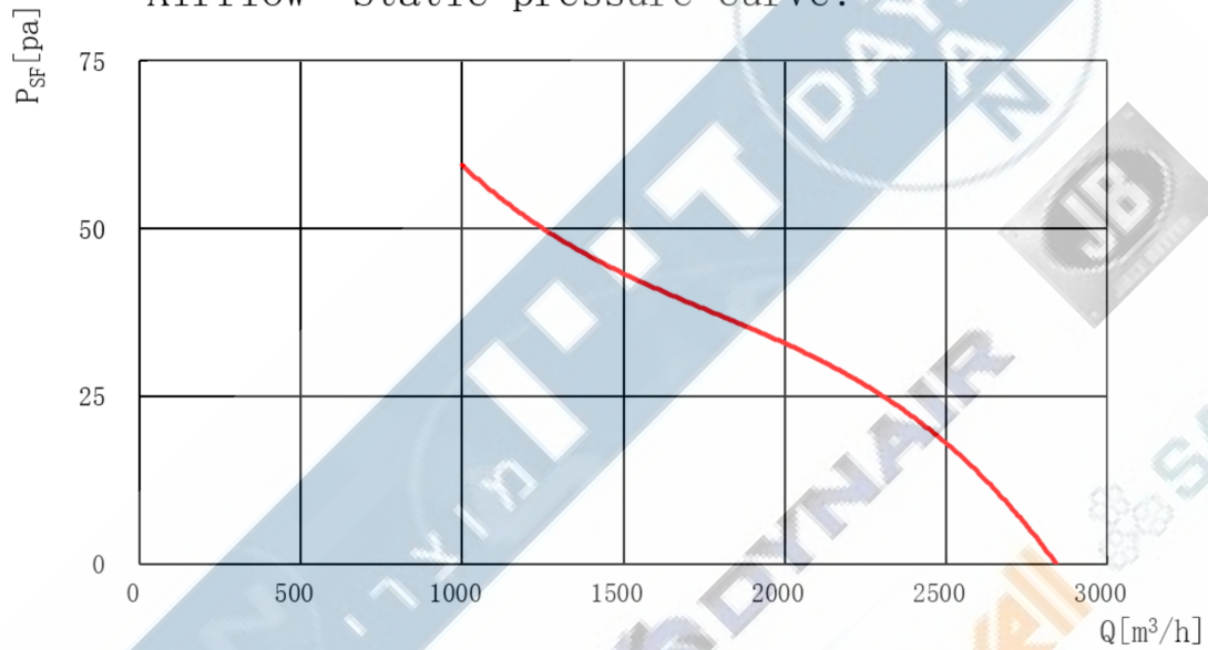
Airflow—Static pressure curve:
