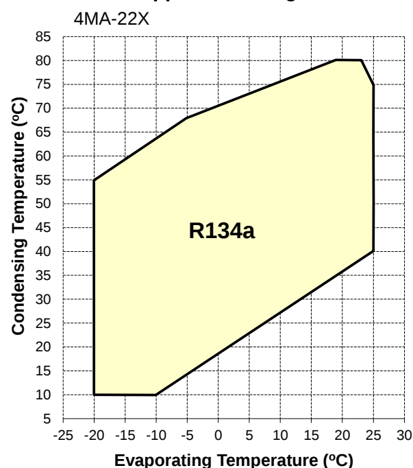
Figure 12: High temp 4M* @ 50% - R134a (1 capacity control)
