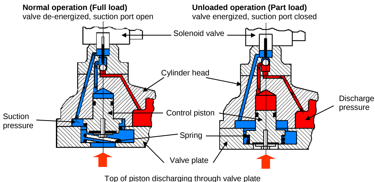
Figure 3: Capacity-controlled operation
