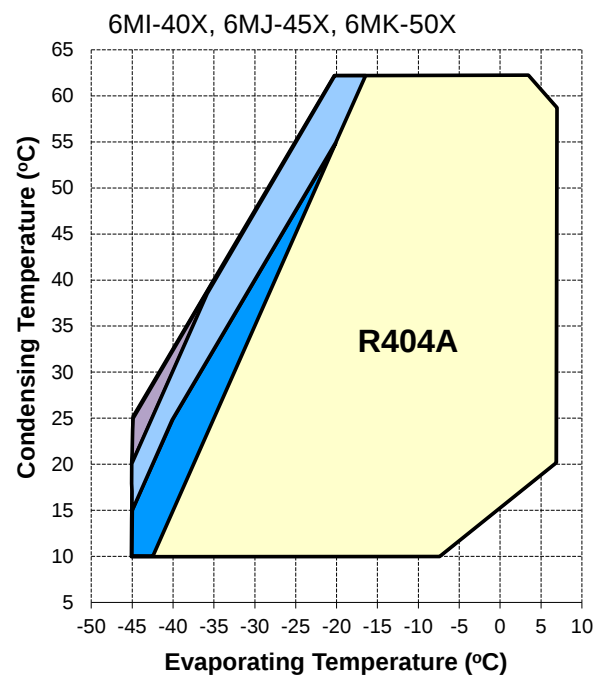
Figure 9: Medium and high temp 6M* @ 33% - R404A (2 capacity controls)
