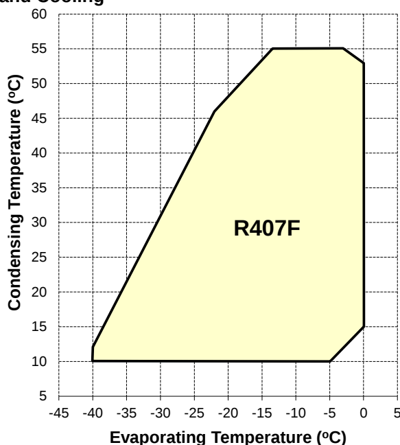
Figure 34: Low and medium temp 6M* @ 33% (2 capacity controls)
