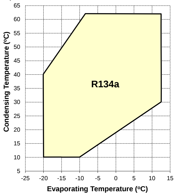
Figure 17: High temp 6M* @ 33% - R134a (2 capacity controls)
