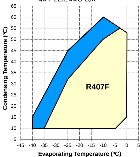
Figure 27: Low and medium temp 4M* @ 50% (1 capacity control)
