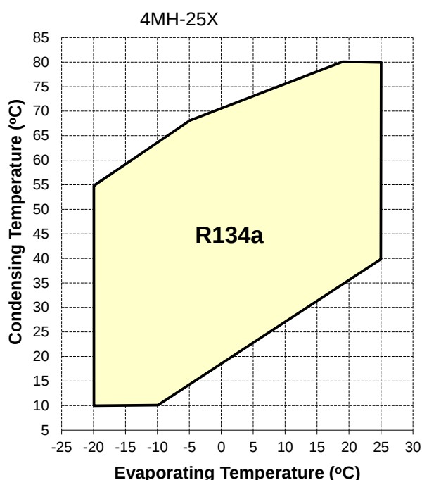
Figure 13: High temp 4M* @ 50% - R134a (1 capacity control)
