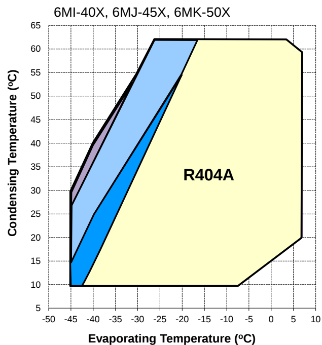
Figure 8: Medium and high temp 6M* @ 66% - R404A (1 capacity control)
