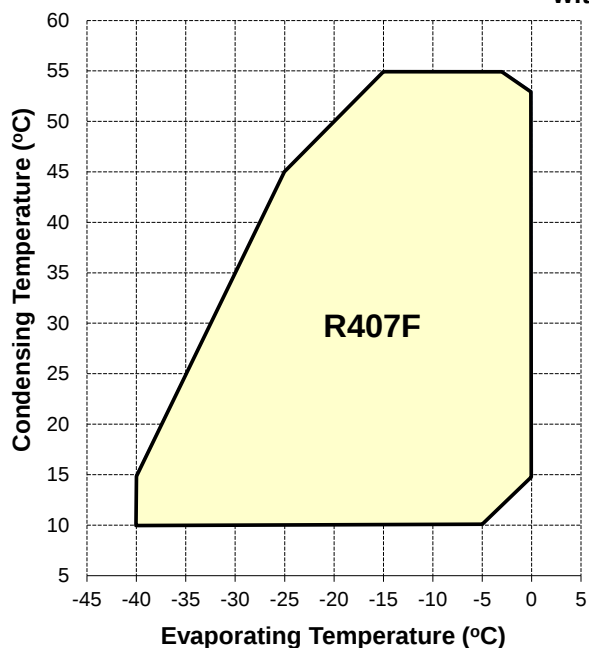
Figure 33: Low and medium temp 6M* @ 66% (1 capacity control)
