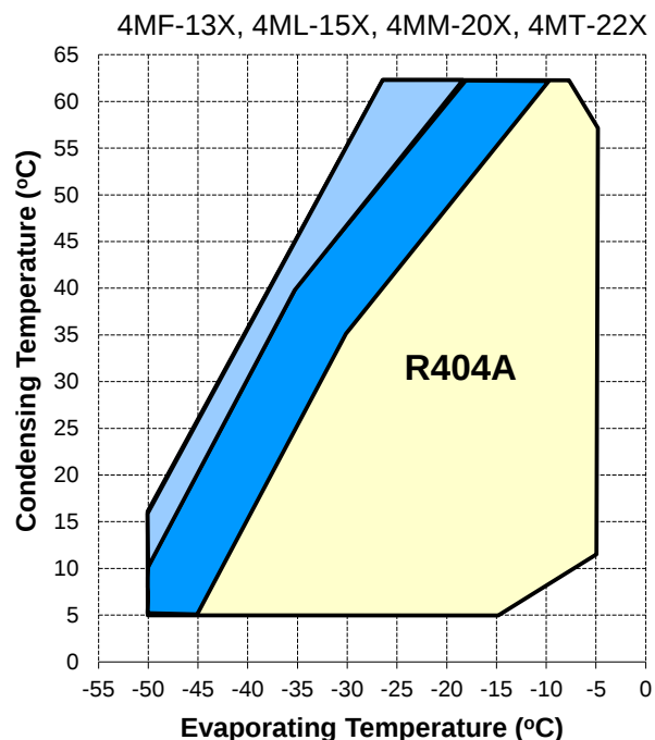
Figure 6: Low and medium temp 4M* @ 50% - R404A (1 capacity control)
