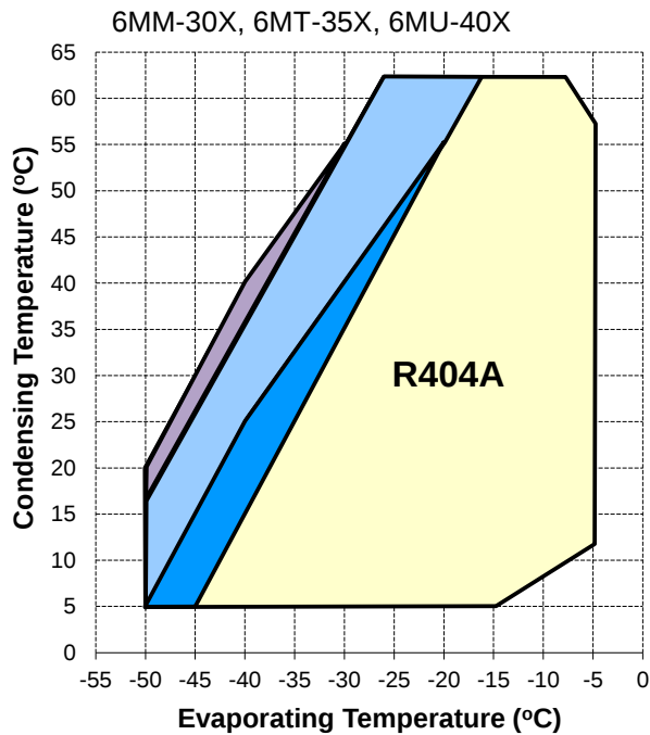
Figure 10: Low and medium temp 6M* @ 66% - R404A (1 capacity control)
