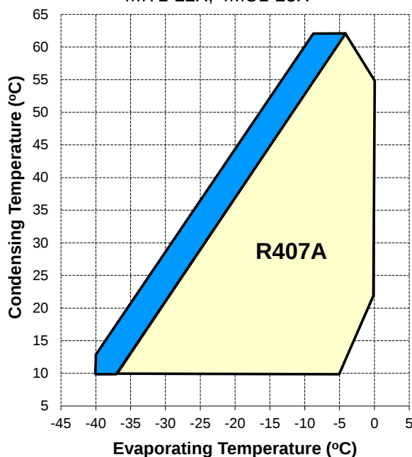
Figure 21: Low and medium temp 4M* @ 50% (1 capacity control)
