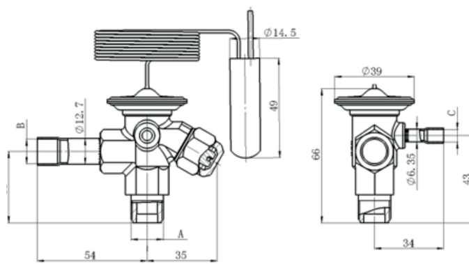
Valve Body - Connection Type: : flare/solder/solder
