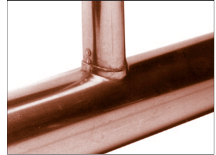
FIGURE 88: Finished joint
