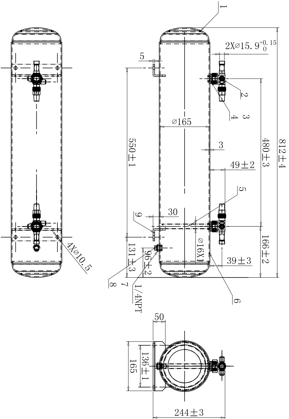
Refrigerant Receiver DHR-800
