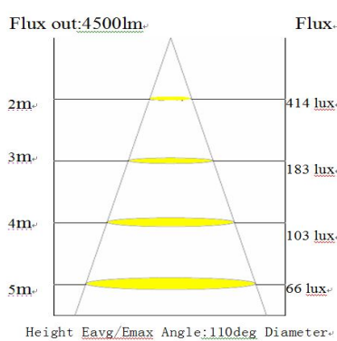
SHF168-AL-50WH 110 degree
