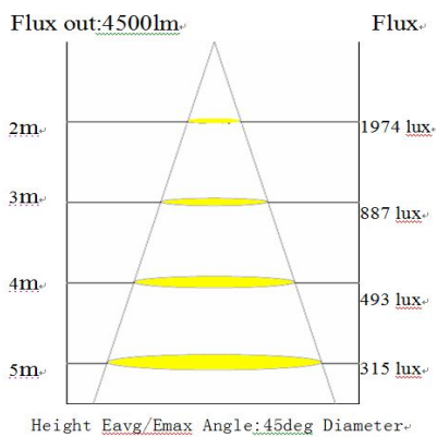
SHF168-AL-50WH 45 degree
