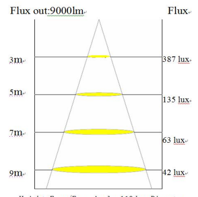
SJF168-AL-120WH 110 degree
