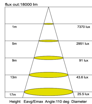
SHF168-AL-200WH 110 degree
