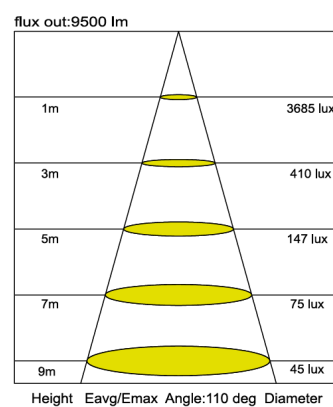
SHF168-AL-100WH 110 degree
