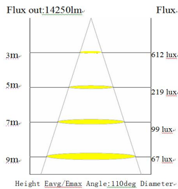
SHF168-AL-150 110 degree
