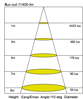
SJF168-AL-120WH 110 degree
