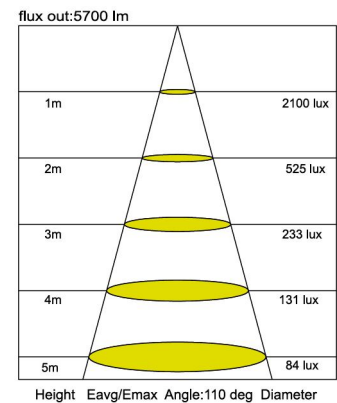
SHF168-AL-60WH 110 degree
