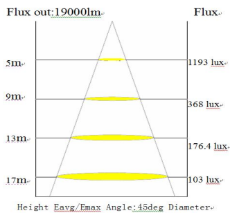
SHF168-AL-200WH
