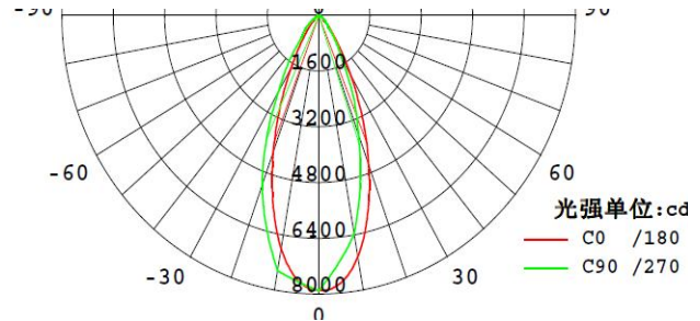
SHF168-AL-50WH 110 degree
