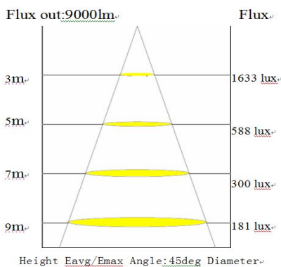
SHF168-AL-95WH 45 degree
