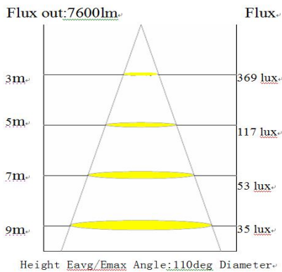
SHF168-AL-80WH 110 degree
