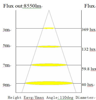
SHF168-AL-90WH 110 degree
