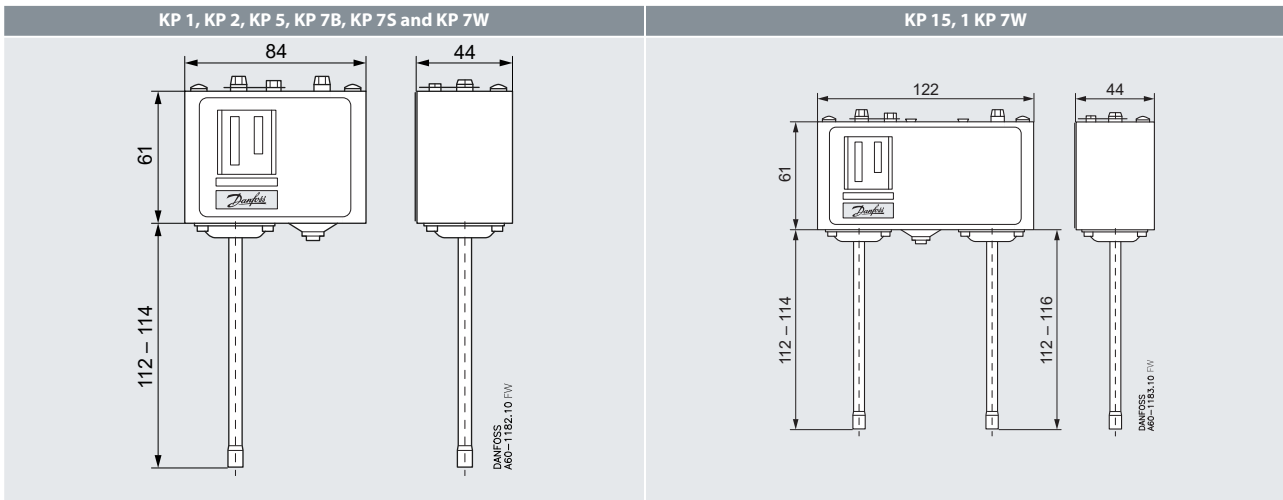
Figure 1: KP with top cover
