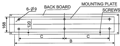
BACK LOOK OF FM□□06
