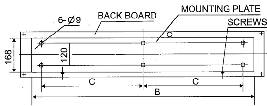
BACK LOOK OF FM□□06
