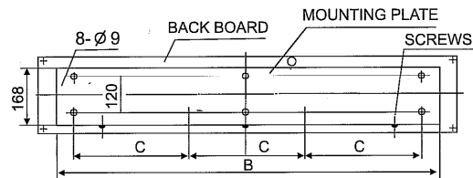
BACK LOOK OF FM□□09, FM□□10, FM□□12, FM□□15, FM□□18
