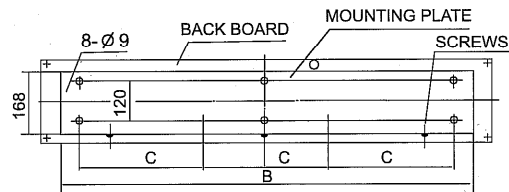
BACK LOOK OF FM□□09, FM□□10, FM□□12, FM□□15, FM□□18
