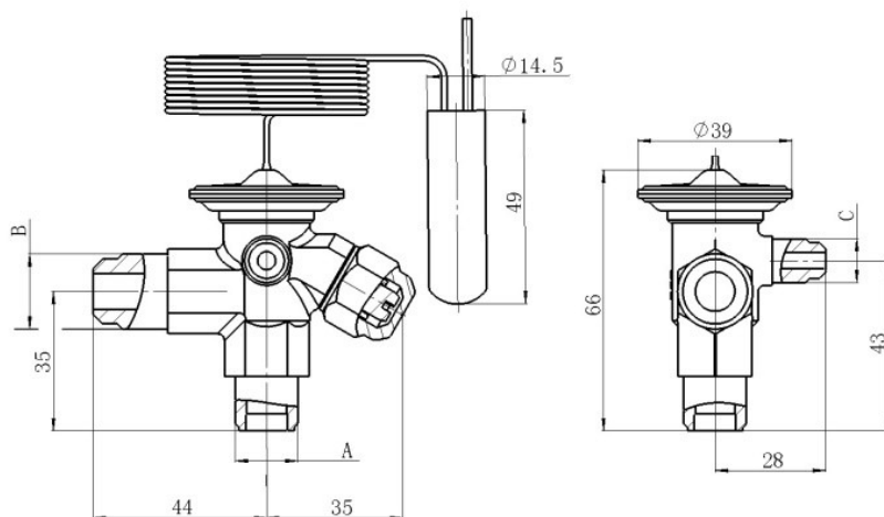
Valve Body - Connection Type: flare/flare/flare
