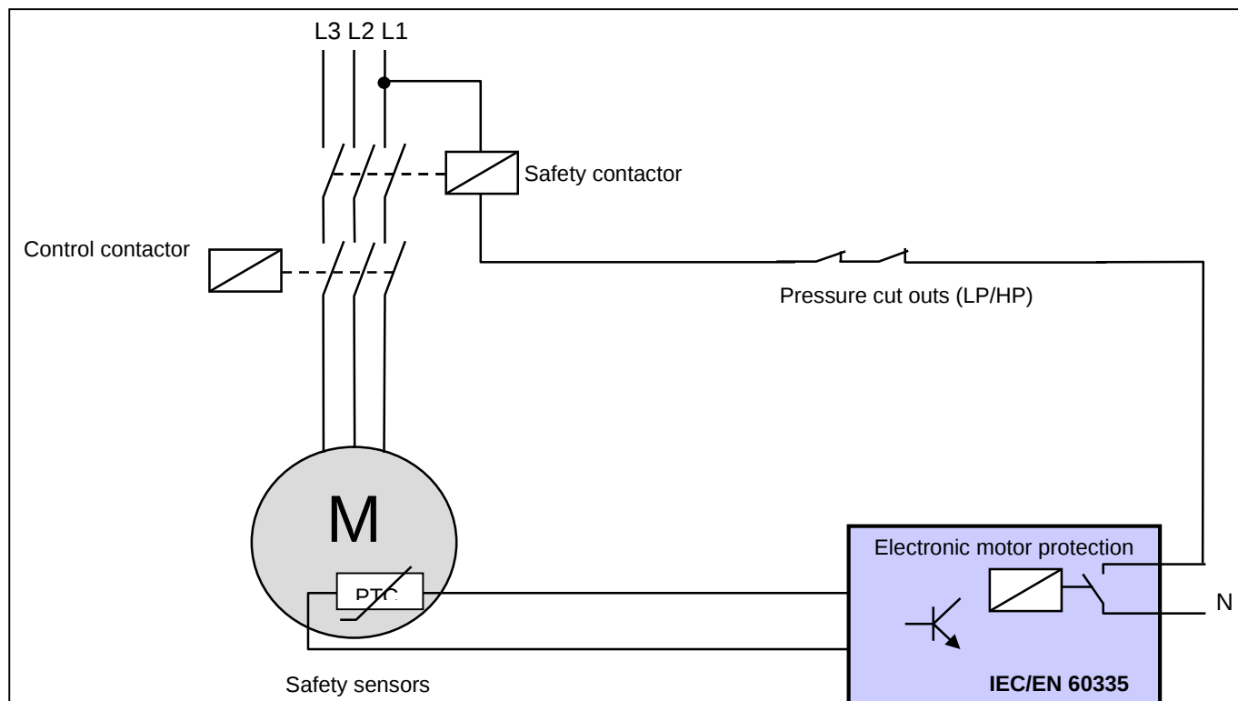
Figure 1: System wiring diagram supporting IEC/EN 60335
